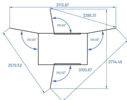
Bottom Fixing & Wiring Holes Diagram
